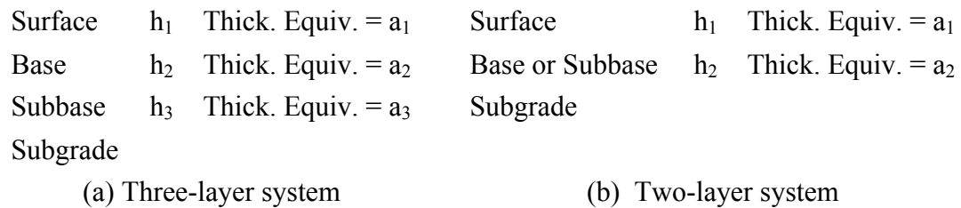
Figure 2. Pavement sections.
