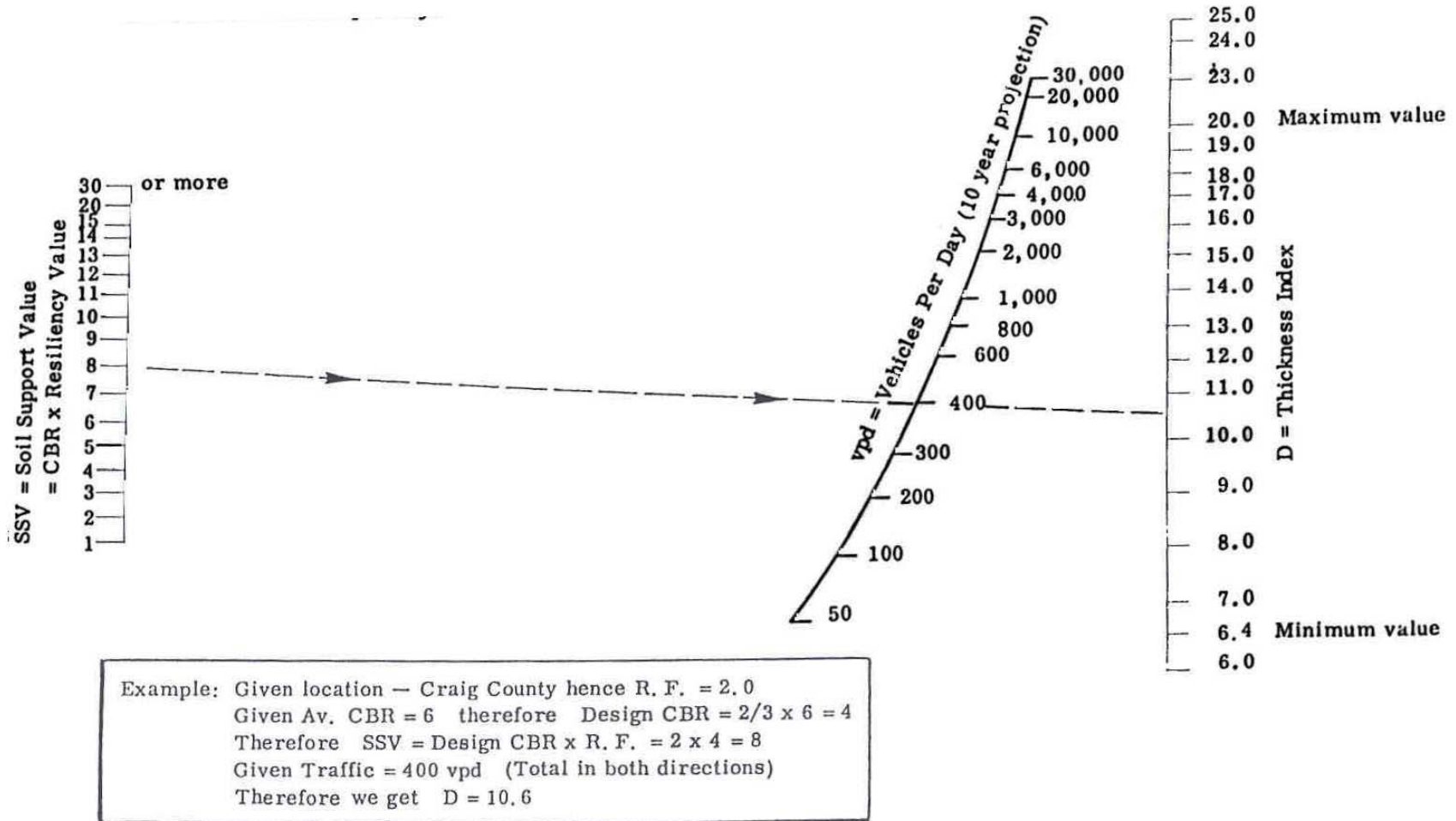
Figure 4 Nomograph correlating the soil support value (SSV), traffic (vpd), and the thickness index (D) (based on AASHO Equation) for subdivision roads.
