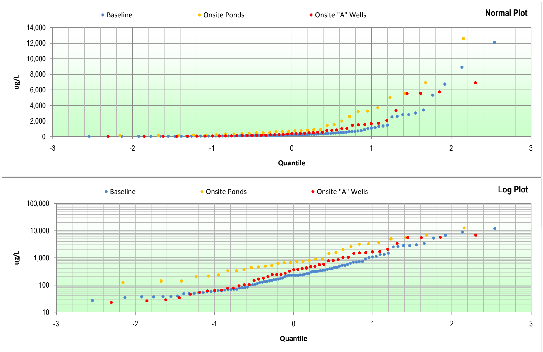
Figure E-16: Aluminum Multiple Quantile Plots Hydrogeologic Investigation and Groundwater Modeling Report Battlefield Golf Club Chesapeake, Virginia
