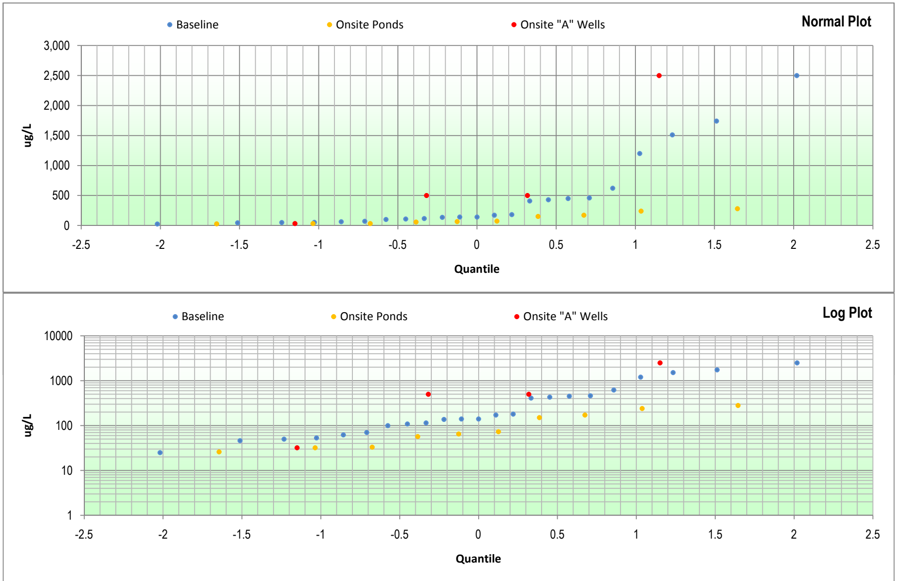
Figure E-27: Nitrate Multiple Quantile Plots Hydrogeologic Investigation and Groundwater Modeling Report Battlefield Golf Club Chesapeake, Virginia
