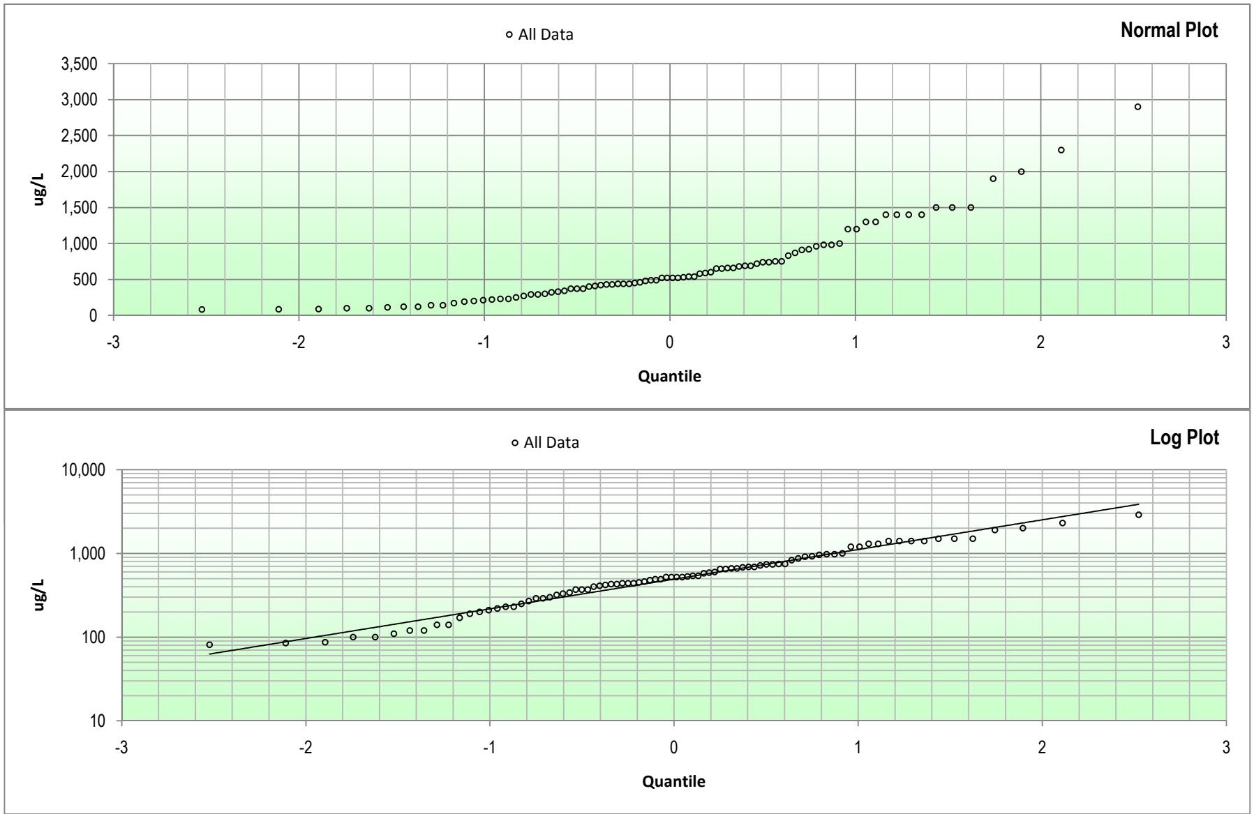
Figure E-2: Ammonia-N Quantile Plots Hydrogeologic Investigation and Groundwater Modeling Report Battlefield Golf Club Chesapeake, Virginia
