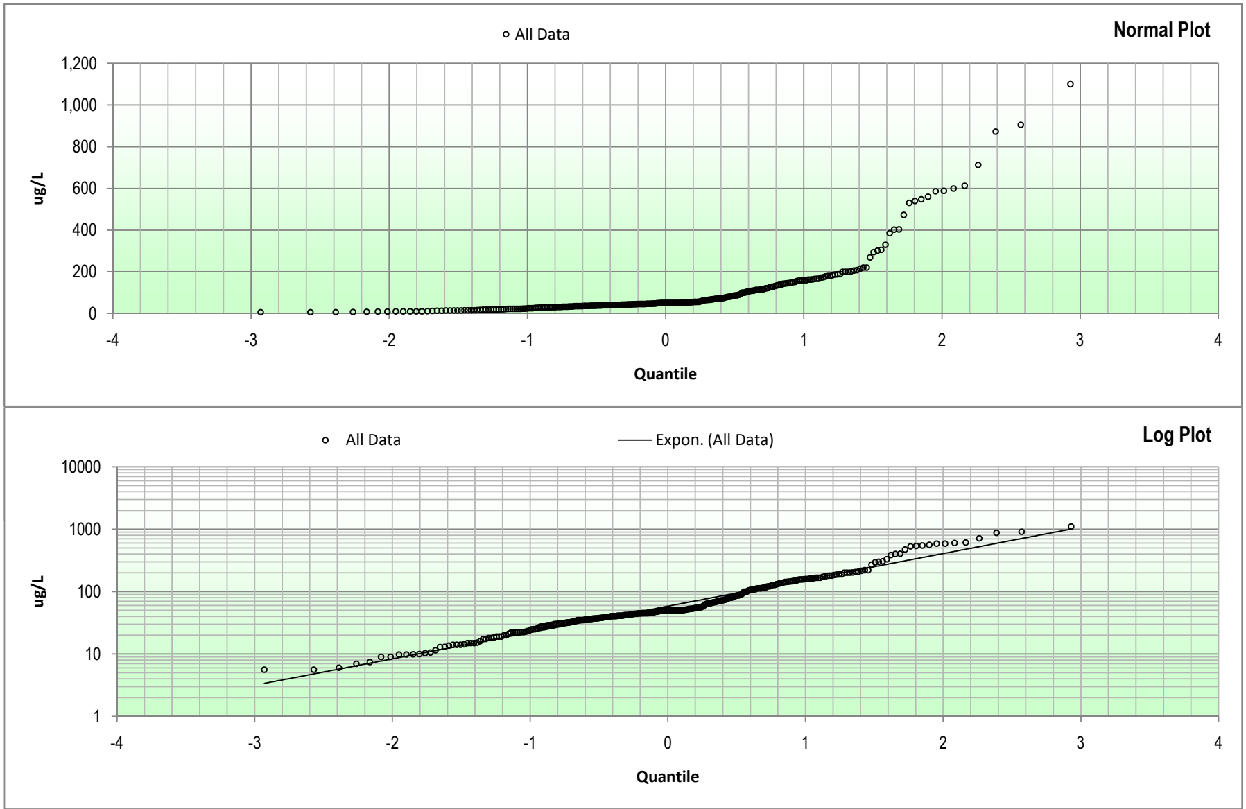
Figure E-5: Boron Quantile Plots Hydrogeologic Investigation and Groundwater Modeling Report Battlefield Golf Club Chesapeake, Virginia
