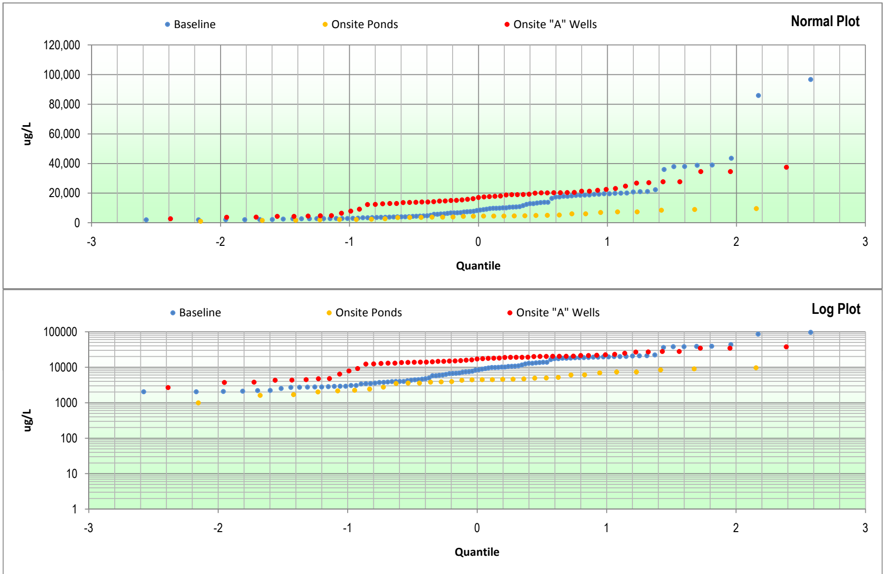
Figure E-24: Magnesium Multiple Quantile Plots Hydrogeologic Investigation and Groundwater Modeling Report Battlefield Golf Club Chesapeake, Virginia
