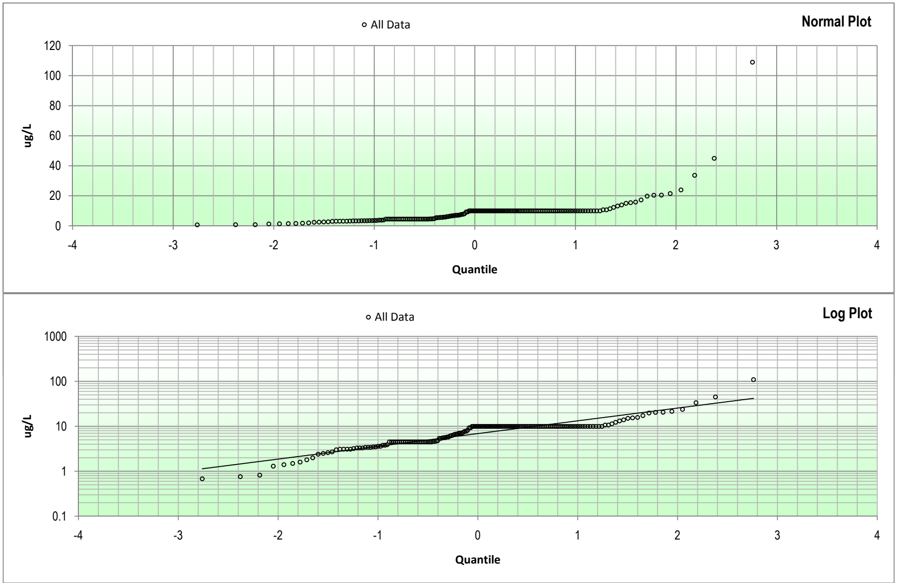
Figure E-3: Arsenic Quantile Plots
