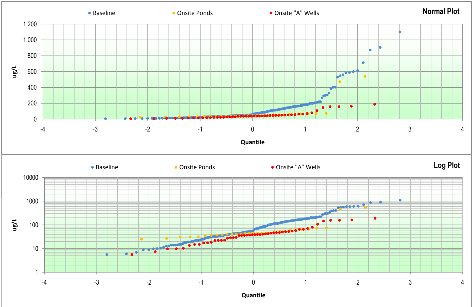
Figure E-20: Boron Multiple Quantile Plots Hydrogeologic Investigation and Groundwater Modeling Report Battlefield Golf Club Chesapeake, Virginia
