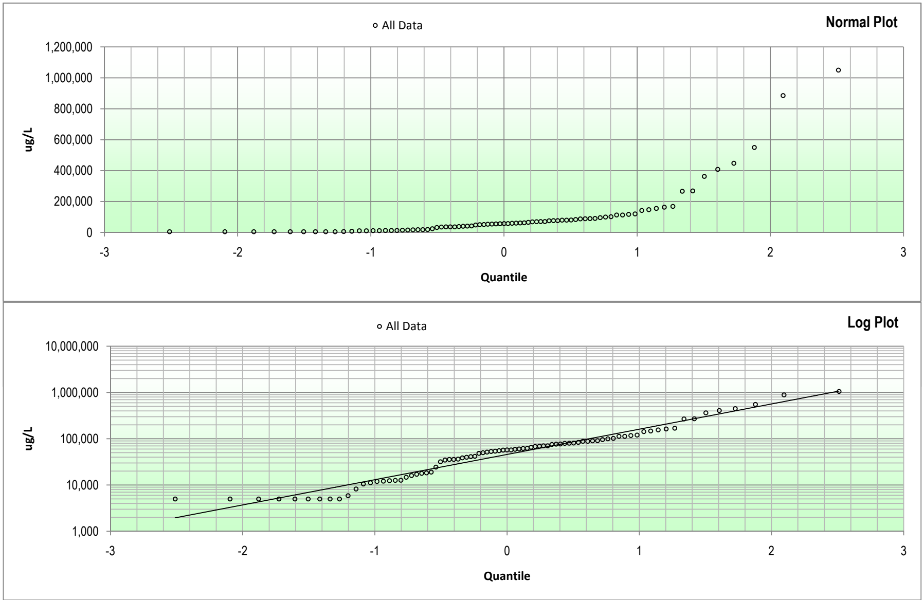
Figure E-14: Sulfate Quantile Plots
