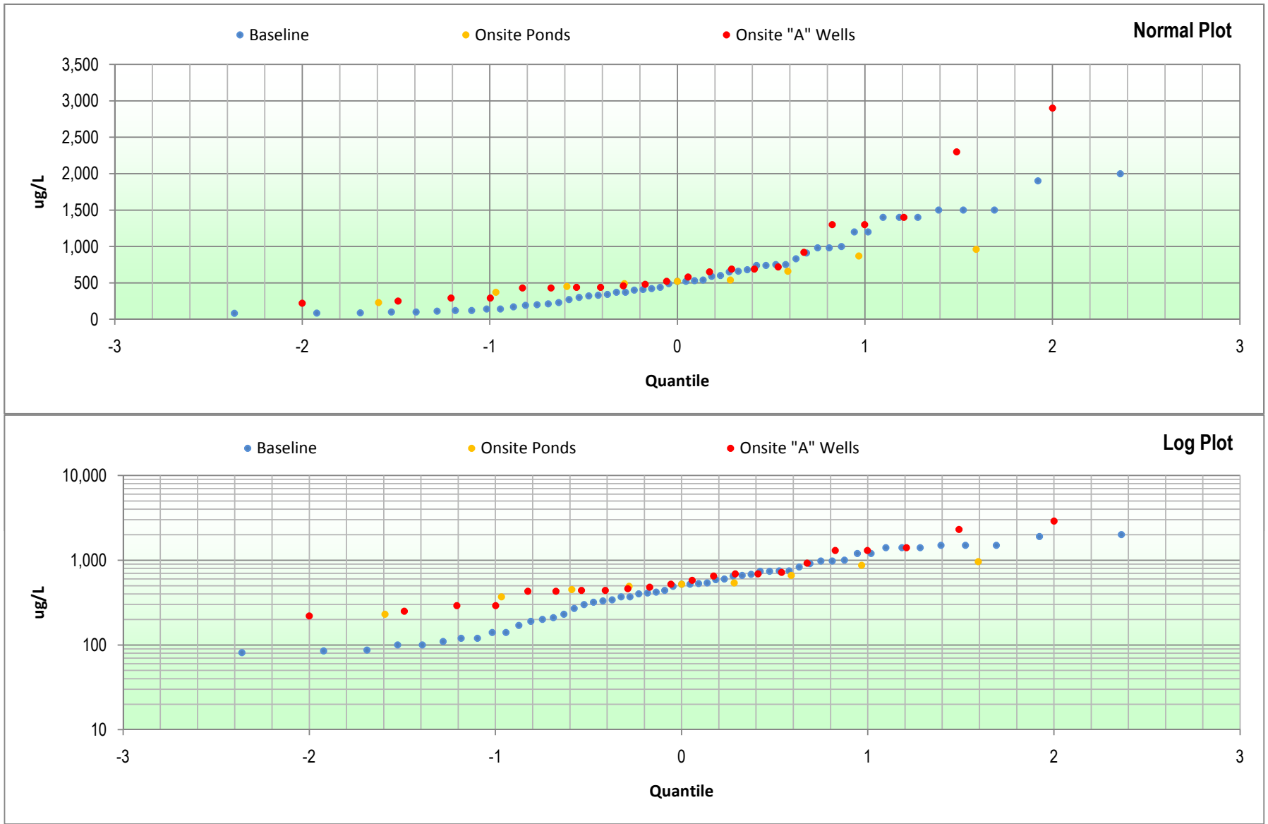
Figure E-17: Ammonia-N Multiple Quantile Plots
