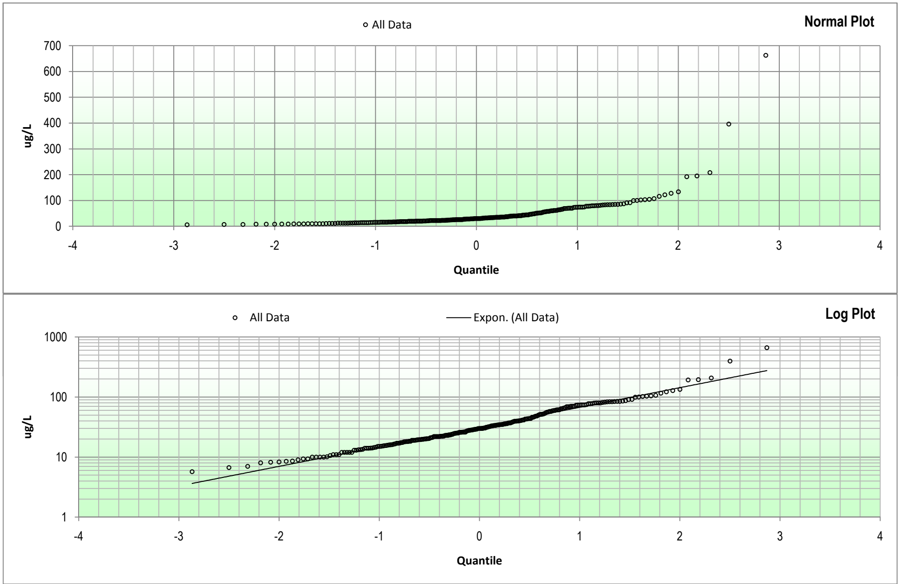
Figure E-4: Barium Quantile Plots
