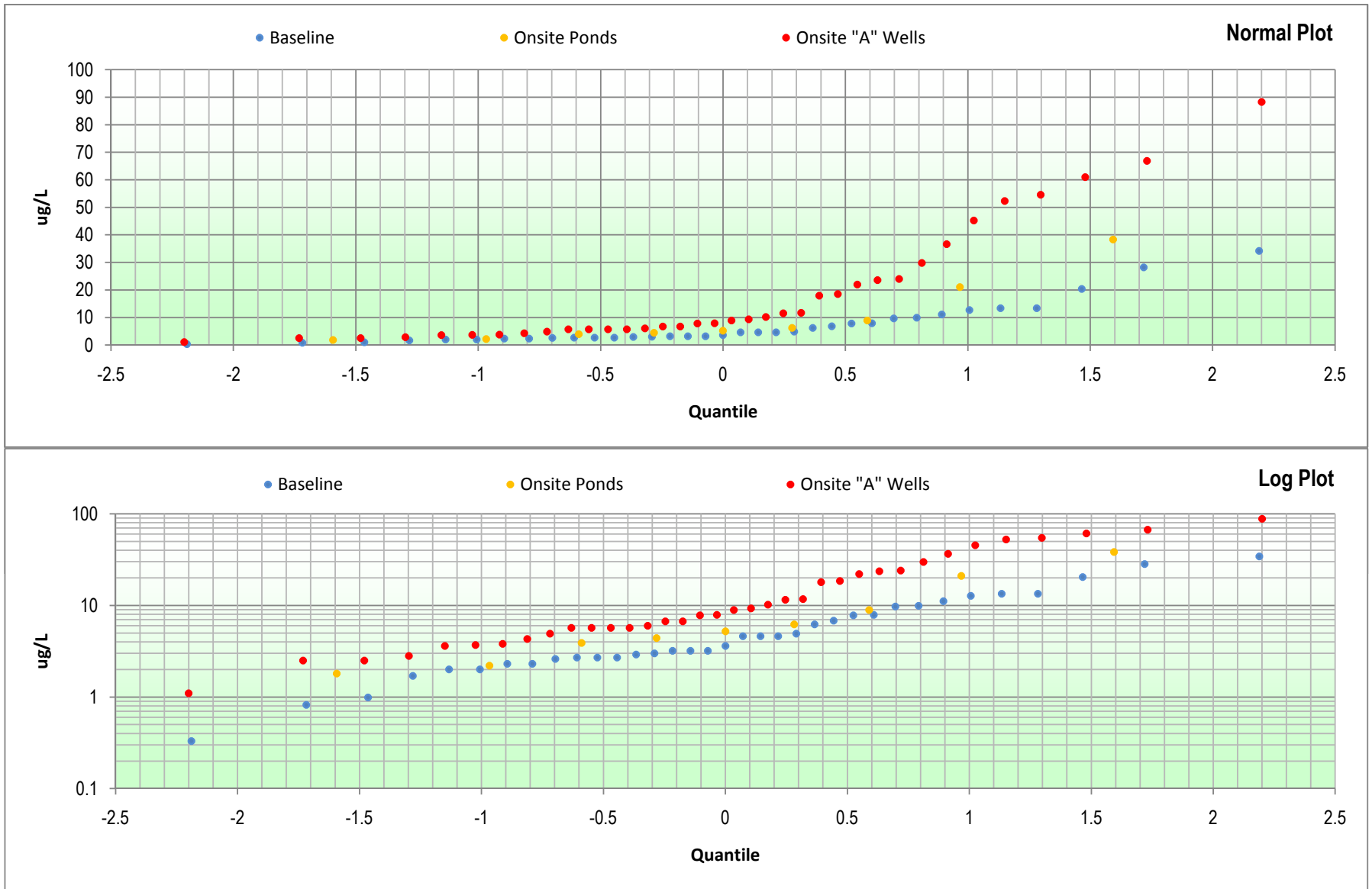
Figure E-26: Nickel Multiple Quantile Plots Hydrogeologic Investigation and Groundwater Modeling Report Battlefield Golf Club Chesapeake, Virginia
