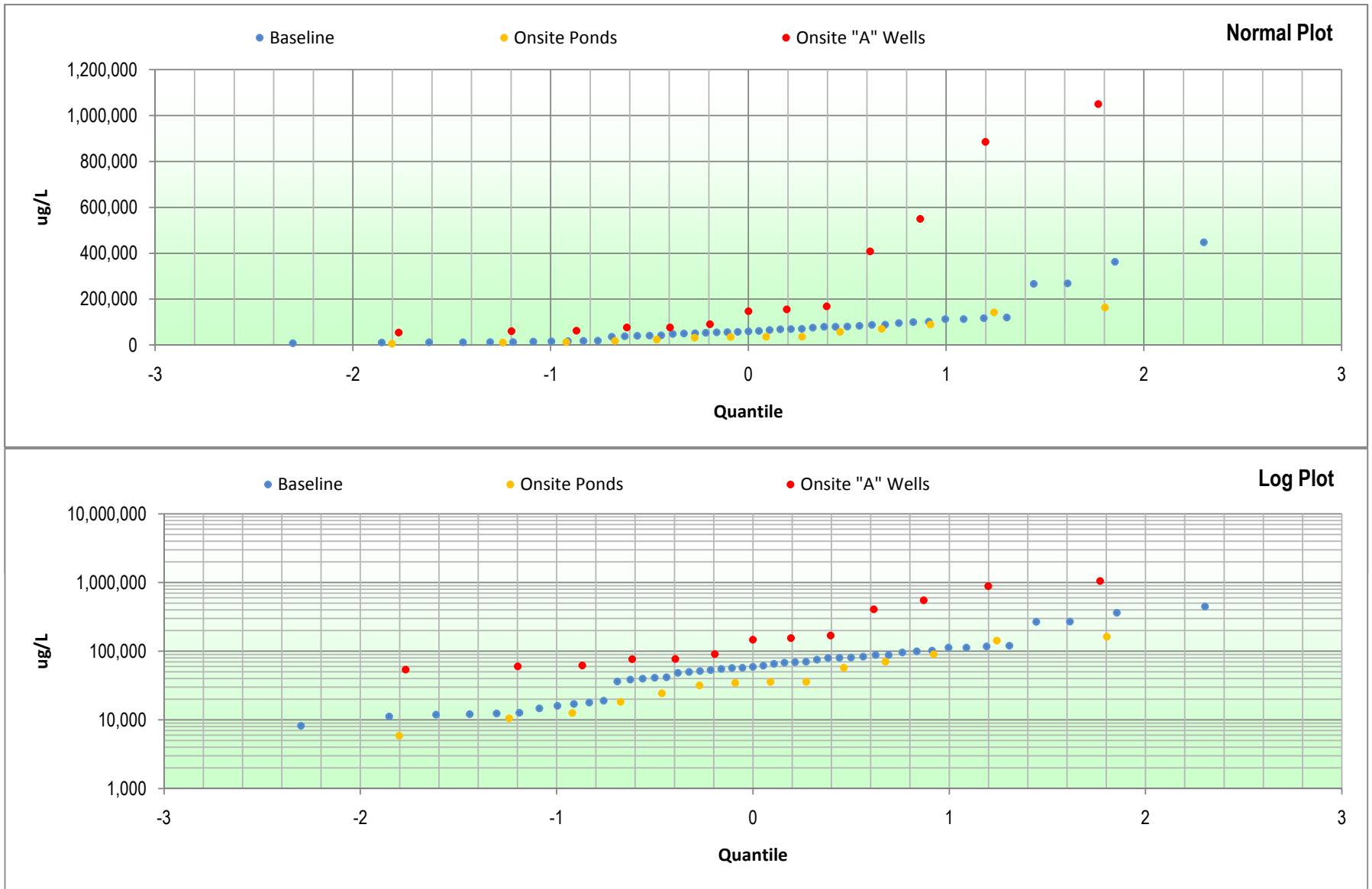
Figure E-29: Sulfate Multiple Quantile Plots Hydrogeologic Investigation and Groundwater Modeling Report Battlefield Golf Club Chesapeake, Virginia
