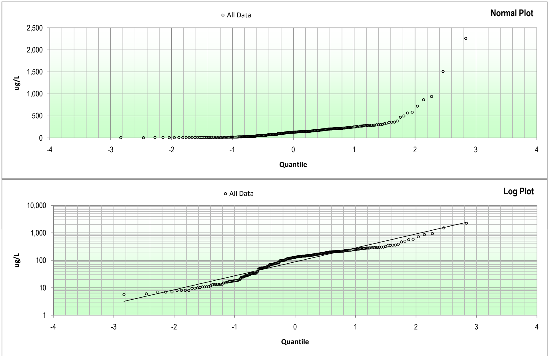
Figure E-10: Manganese Quantile Plots
