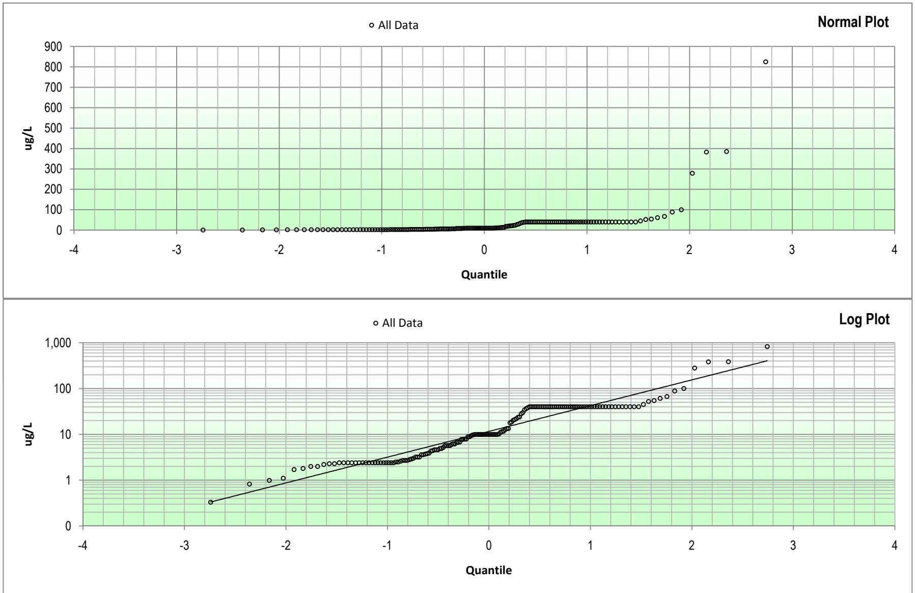
Figure E-11: Nickel Quantile Plots
