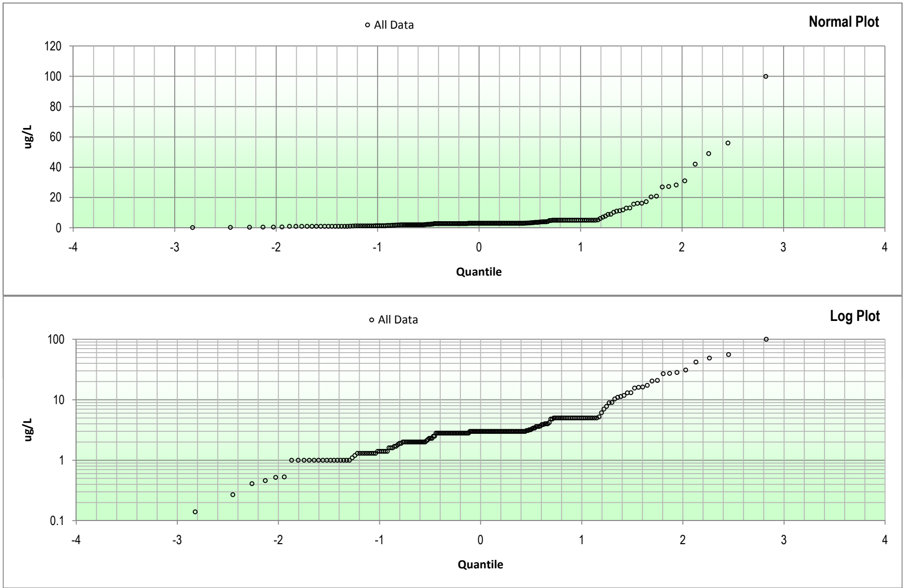
Figure E-8: Lead Quantile Plots
