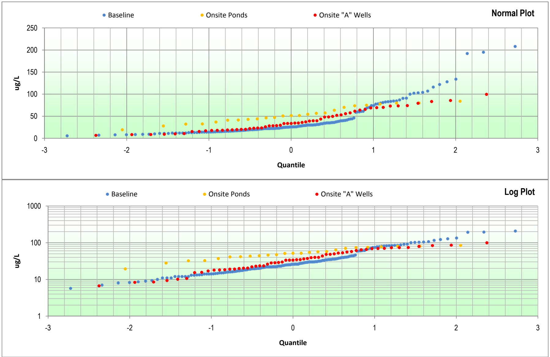
Figure E-19: Barium Multiple Quantile Plots Hydrogeologic Investigation and Groundwater Modeling Report Battlefield Golf Club Chesapeake, Virginia
