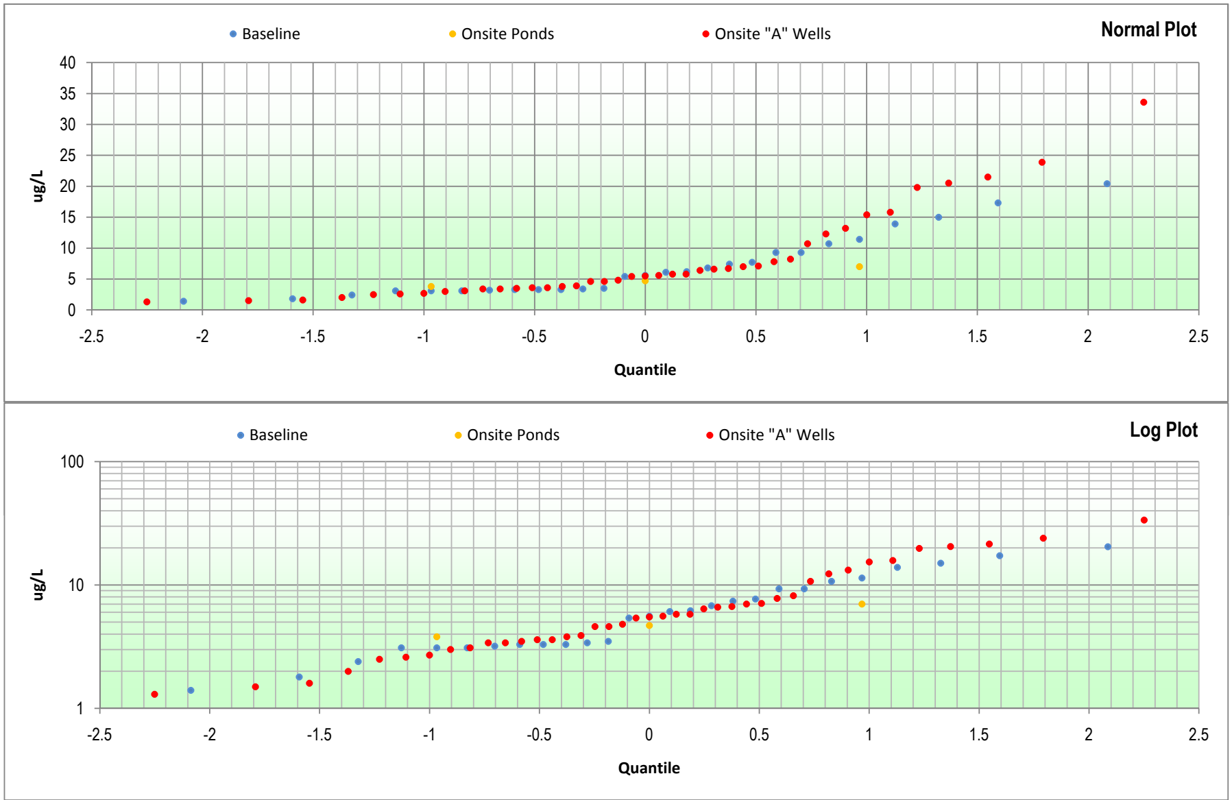
Figure E-18: Arsenic Multiple Quantile Plots Hydrogeologic Investigation and Groundwater Modeling Report Battlefield Golf Club Chesapeake, Virginia
