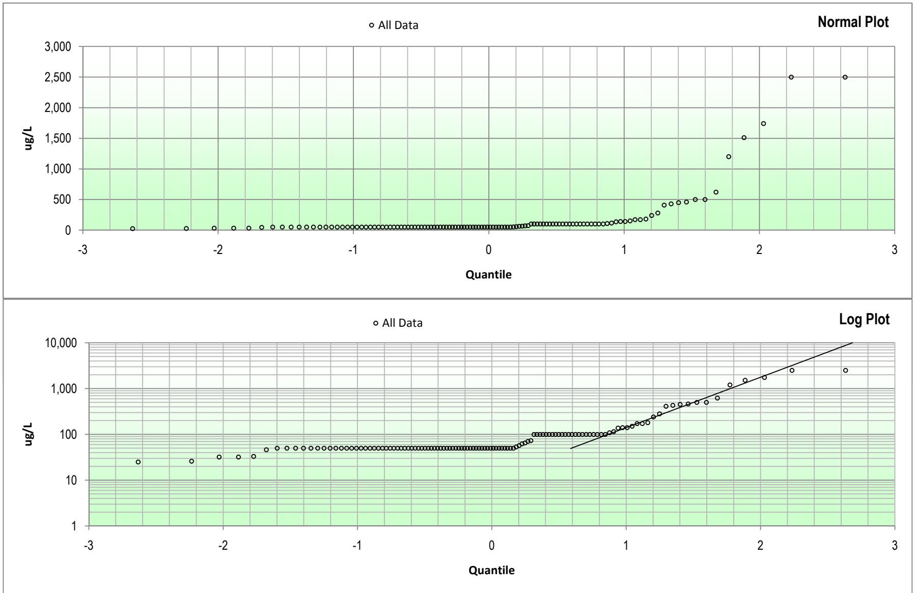
Figure E-12: Nitrate Quantile Plots
