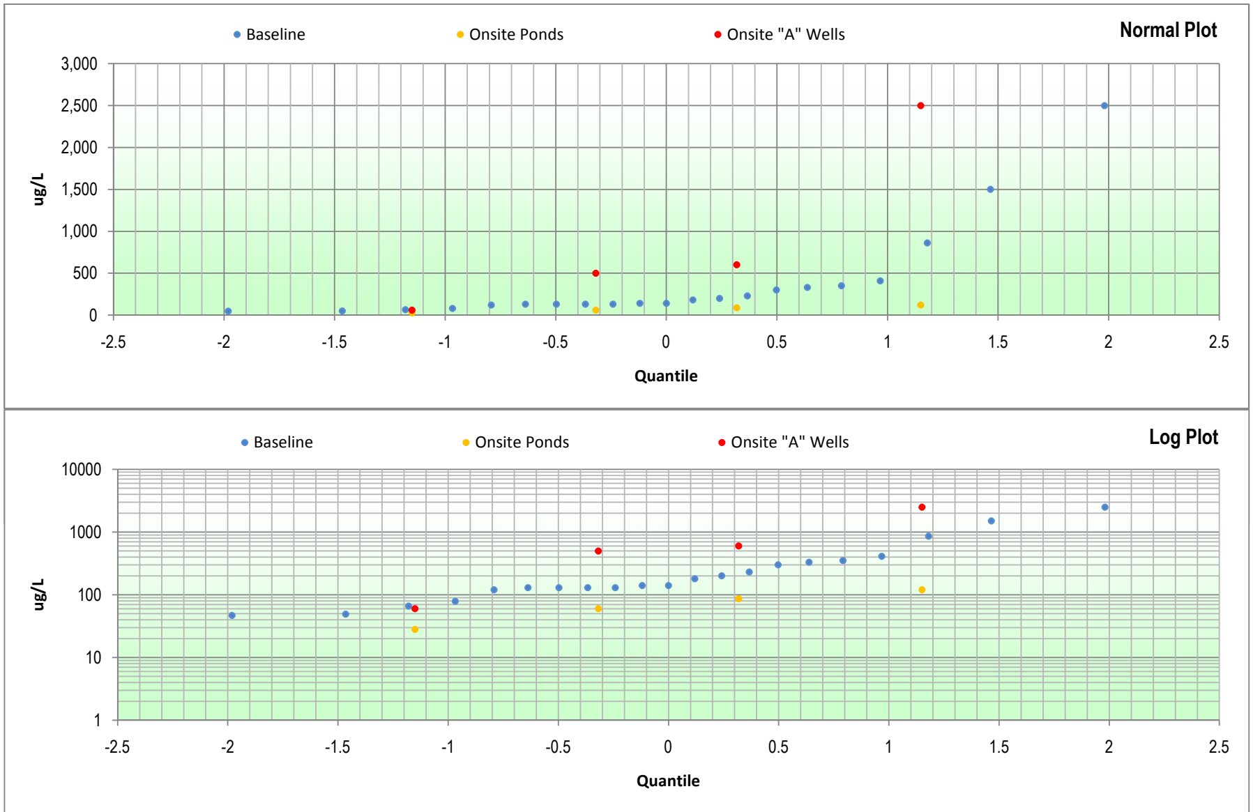
Figure E-28: Nitrite Multiple Quantile Plots Hydrogeologic Investigation and Groundwater Modeling Report Battlefield Golf Club Chesapeake, Virginia
