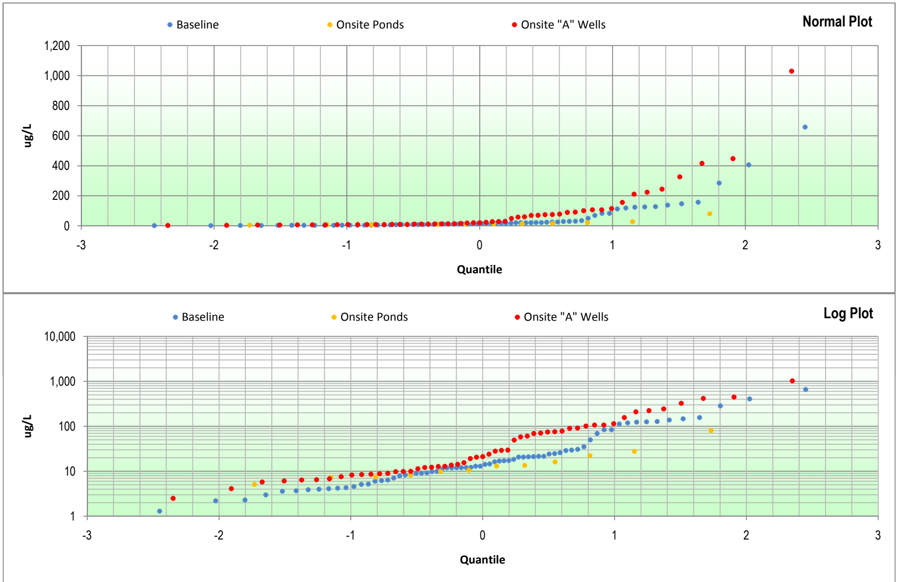
Figure E-30: Zinc Multiple Quantile Plots Hydrogeologic Investigation and Groundwater Modeling Report Battlefield Golf Club Chesapeake, Virginia
