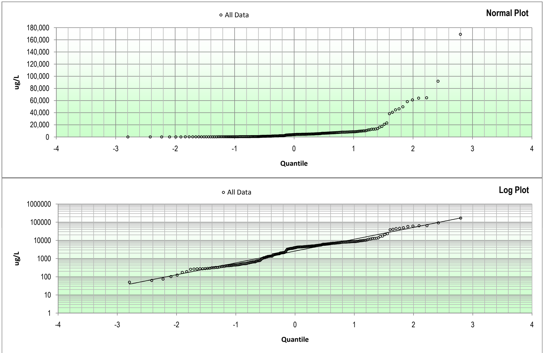
Figure E-7: Iron Quantile Plots
