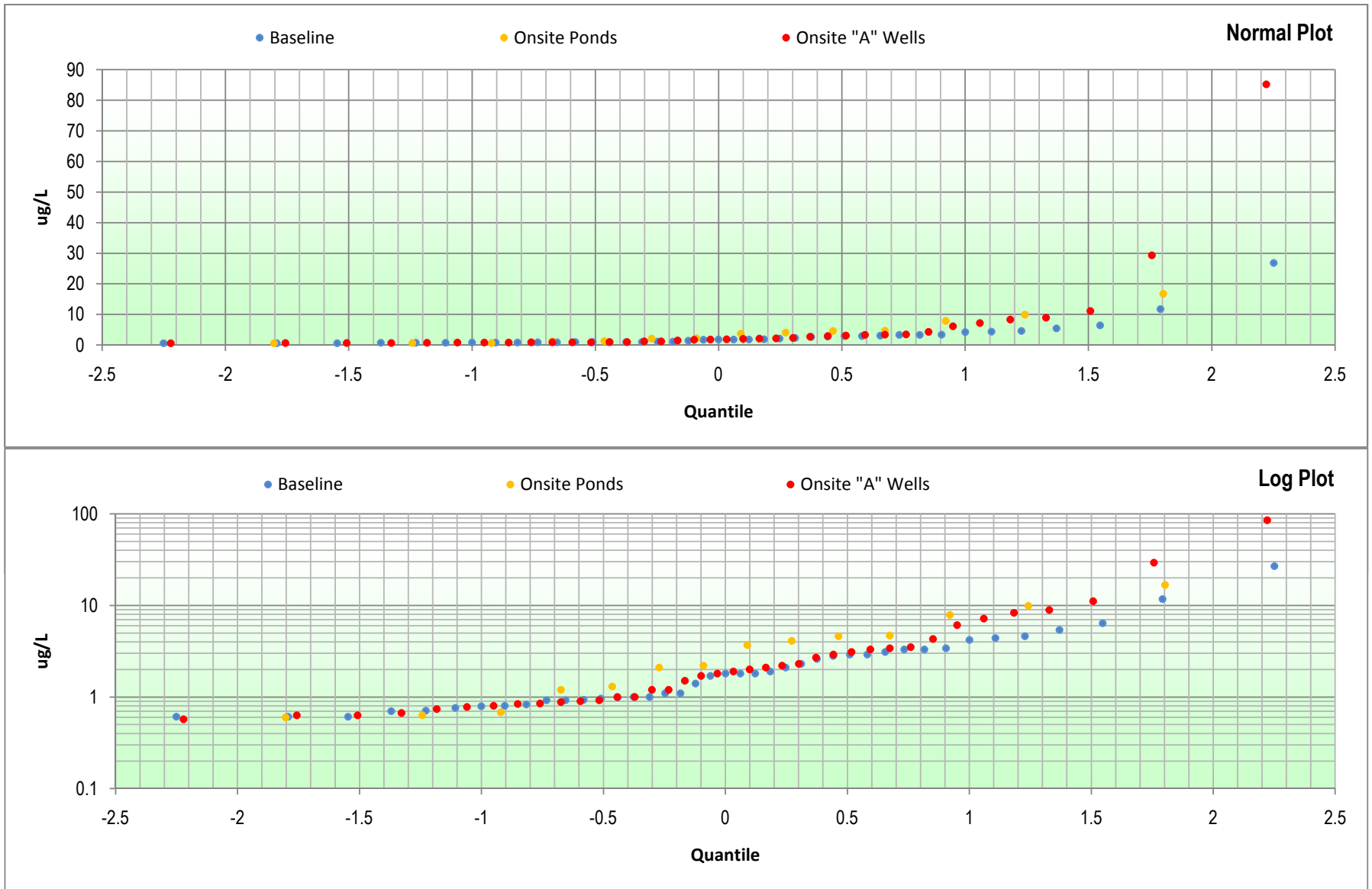
Figure E-21: Chromium Multiple Quantile Plots Hydrogeologic Investigation and Groundwater Modeling Report Battlefield Golf Club Chesapeake, Virginia
