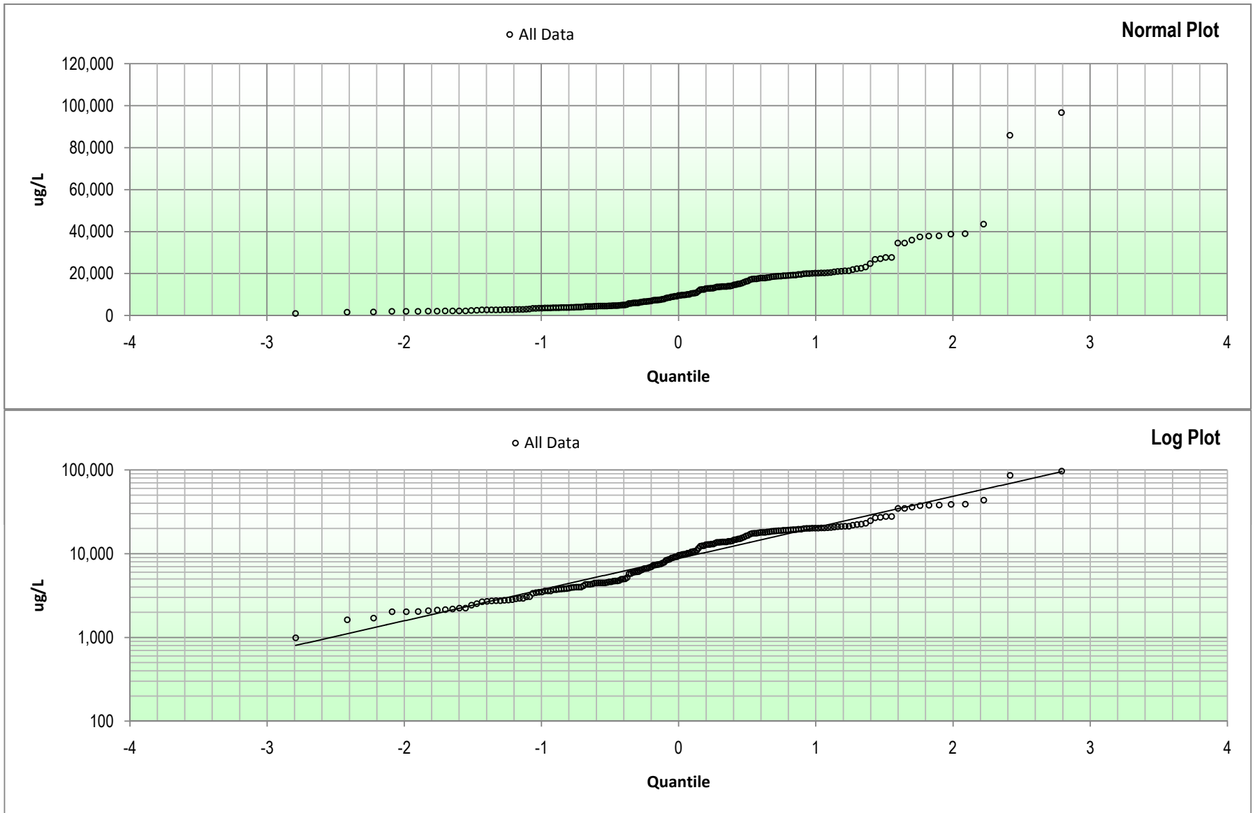
Figure E-9: Magnesium Quantile Plots
