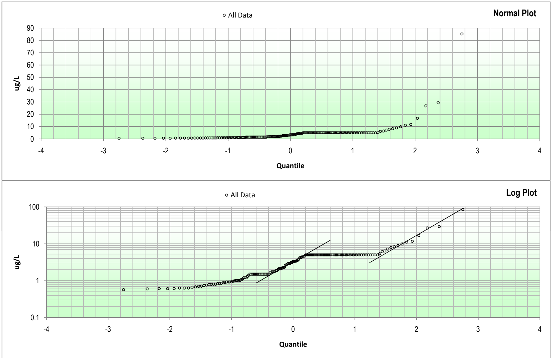
Figure E-6: Chromium Quantile Plots
