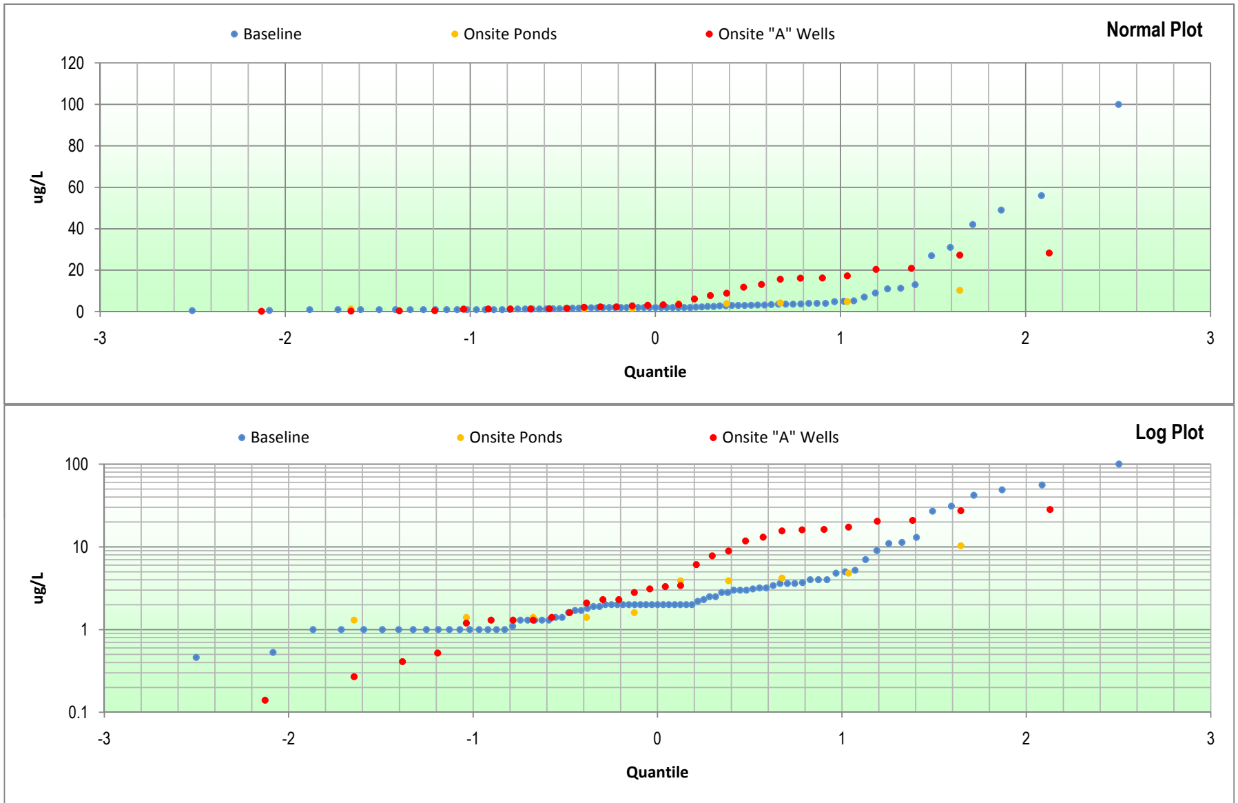
Figure E-23: Lead Multiple Quantile Plots Hydrogeologic Investigation and Groundwater Modeling Report Battlefield Golf Club Chesapeake, Virginia
