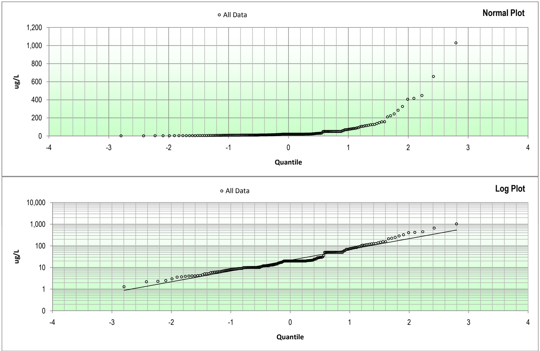
Figure E-15: Zinc Quantile Plots
