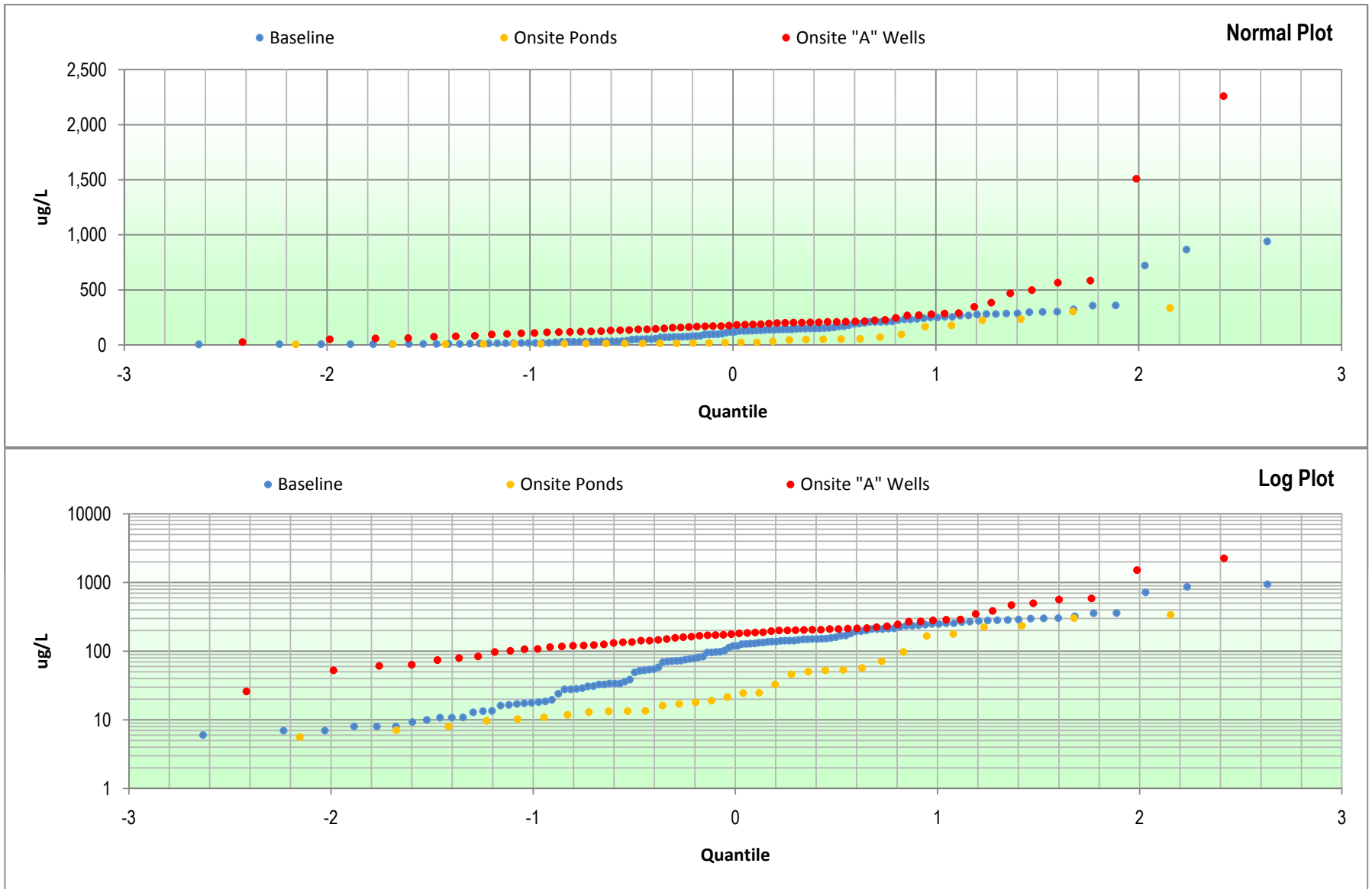
Figure E-25: Manganese Multiple Quantile Plots Hydrogeologic Investigation and Groundwater Modeling Report Battlefield Golf Club Chesapeake, Virginia
