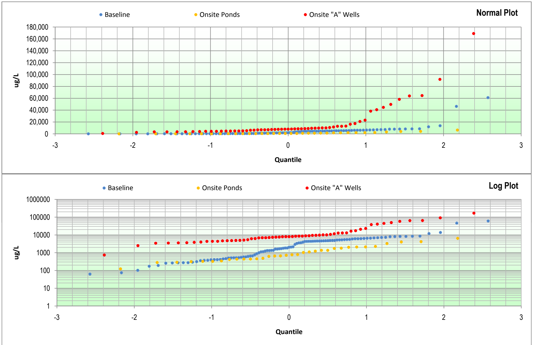
Figure E-22: Iron Multiple Quantile Plots Hydrogeologic Investigation and Groundwater Modeling Report Battlefield Golf Club Chesapeake, Virginia
