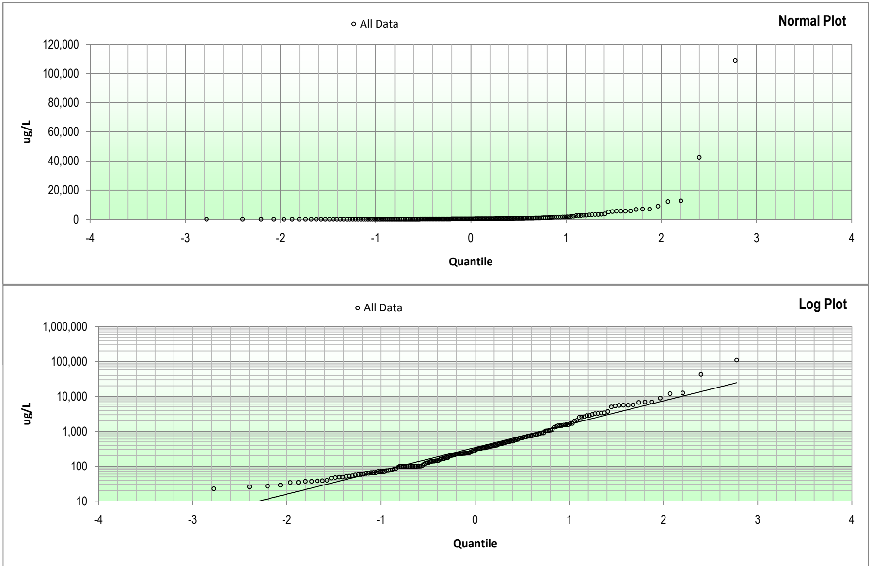
Figure E-1: Aluminum Quantile Plots
