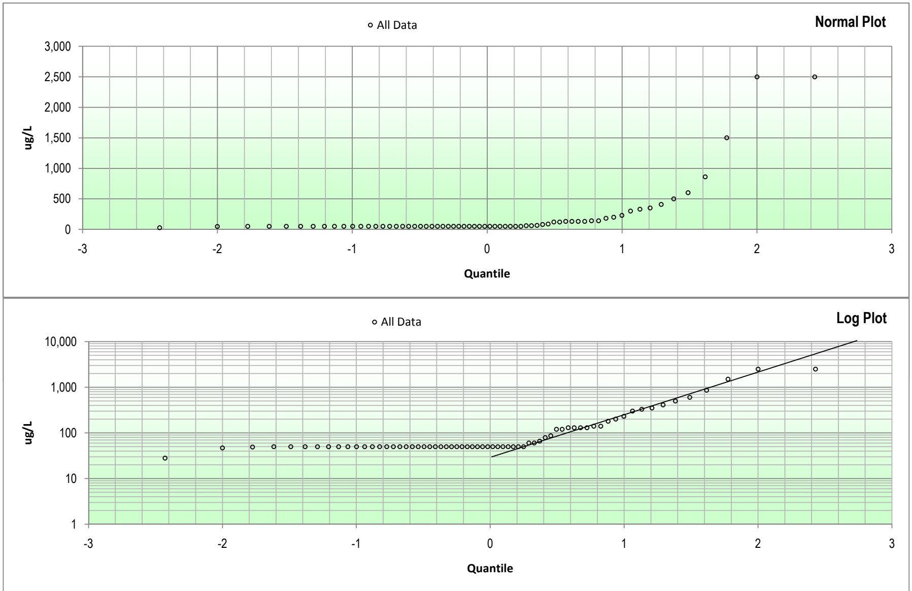
Figure E-13: Nitrite Quantile Plots
